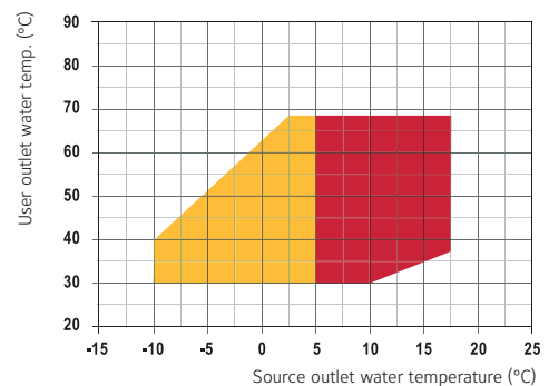
Operation limits LT version
