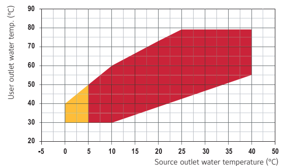
Operation limits LT version
