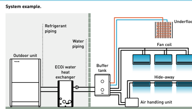
A buffer tank of minimum 280 l for 28 kW and 500 l for 50 kW is always needed.
