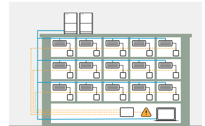
Fig 2: Standalone leak detection system.
