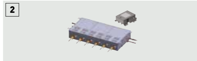
2 3-Pipe control box kit. Heat Recovery box to connect multiple indoor units with just one box, 4, 6 and up to 8 indoor units or groups. This is good advantage in the restaurants, where space for connecting several boxes is limited.
